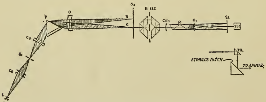
FIG. 5. GROUND PLAN DOUBLE SPECTROMETER
